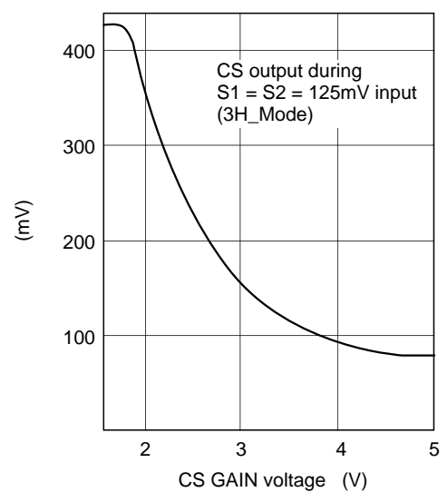
CS GAIN control characteristics
