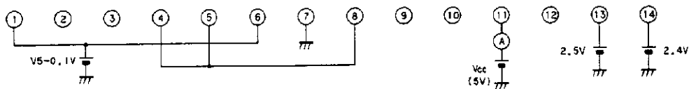
Pin ⑪ current test
