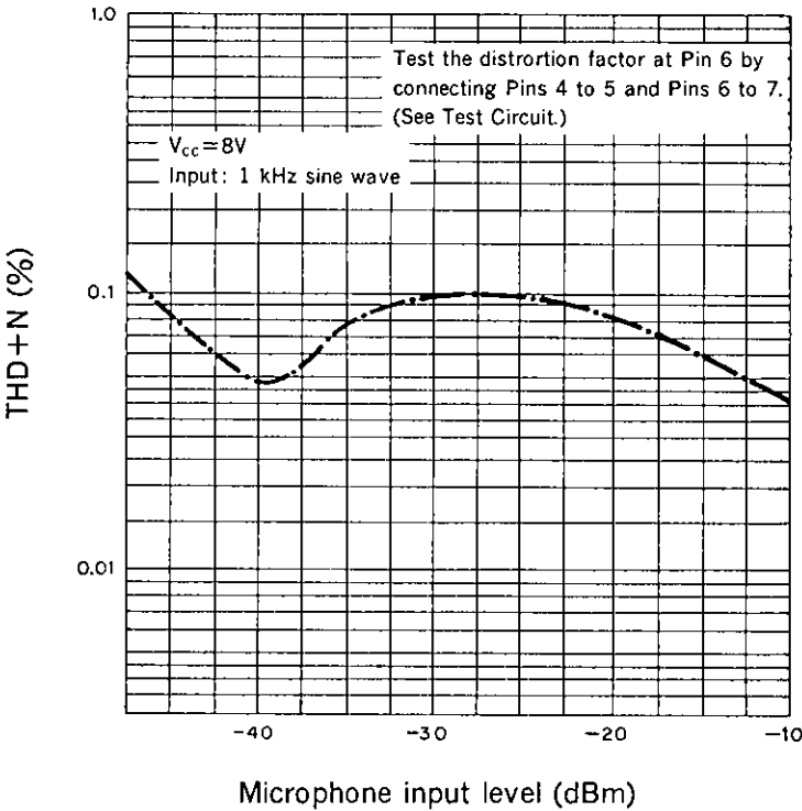
AGC Total Harmonic Distortion Factor
