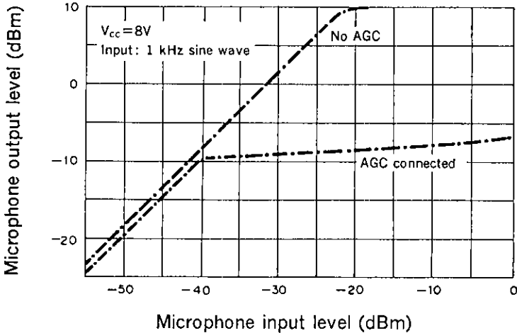
Microphone Output Voltage Characteristics
