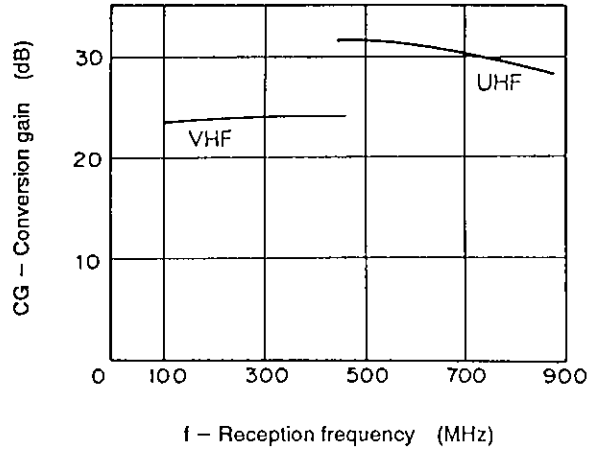
Conversion Gain vs. Reception Frequency (Untuned Input) Input level is -40dBm
