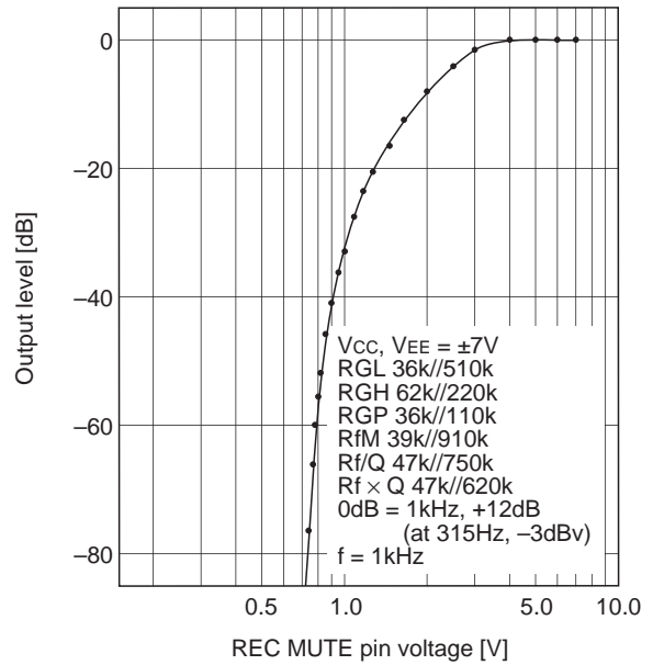
Output level vs. Mute characteristics 3
