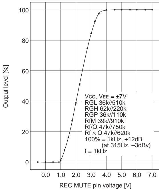
Output level vs. Mute characteristics 1
