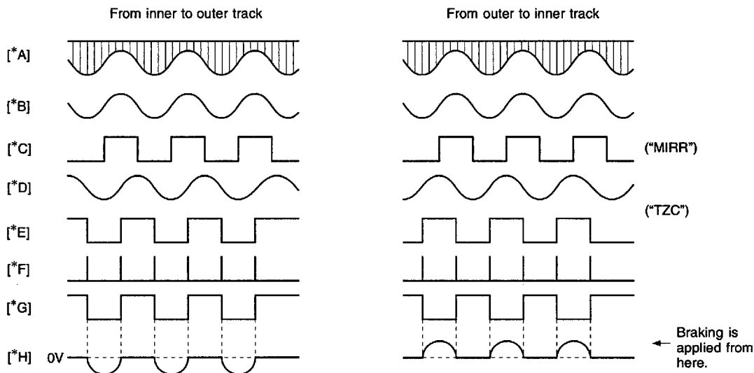
Fig. 7. Internal waveform
