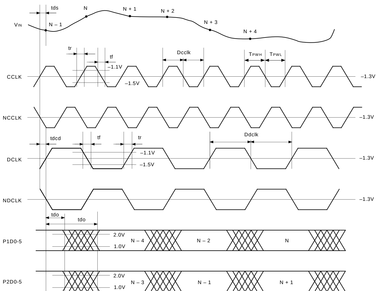
Timing Chart 1
