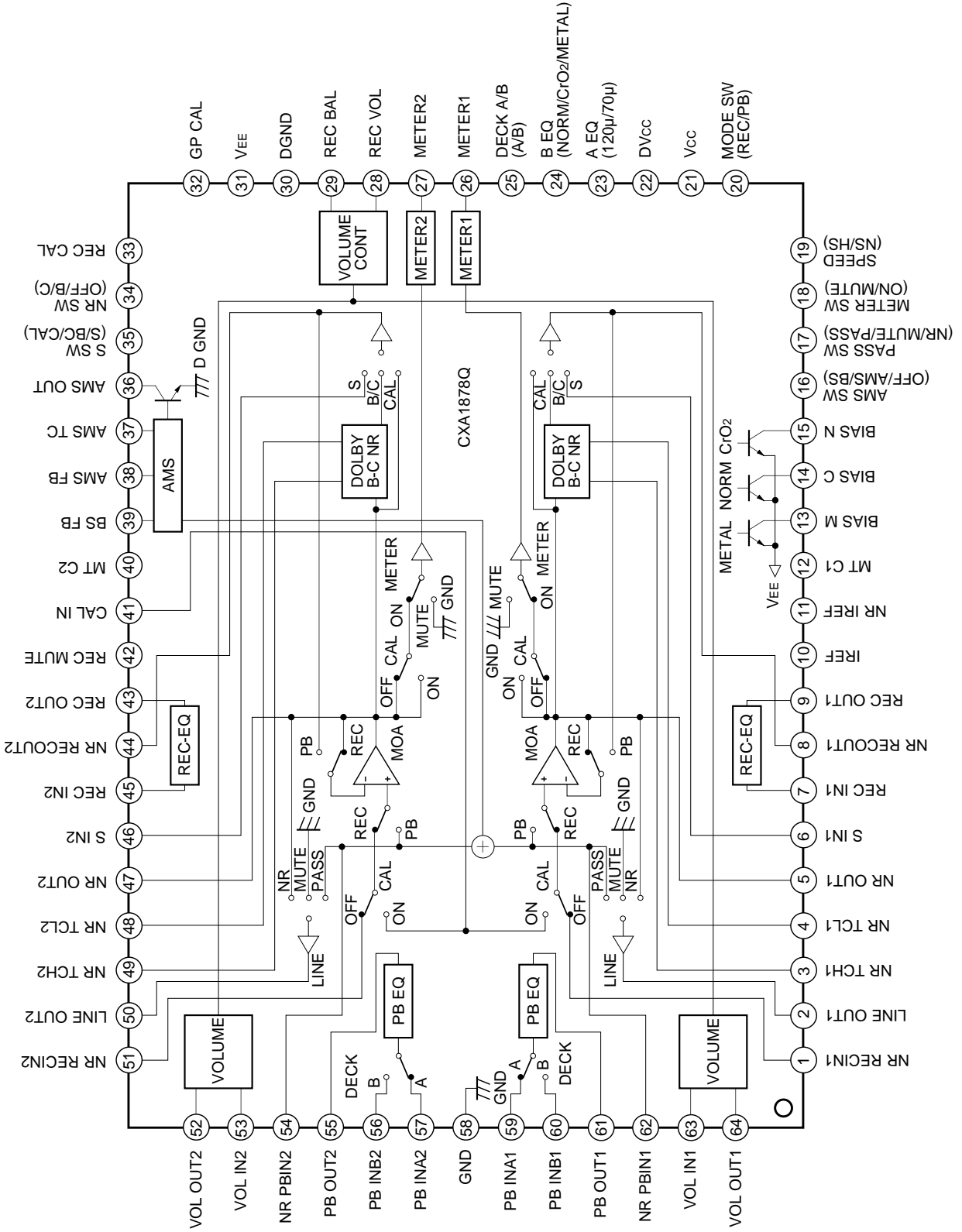
Block Diagram and Pin Configuration
