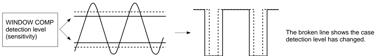
Fig. 5. Conceptual diagram of WINDOW comparator operation
