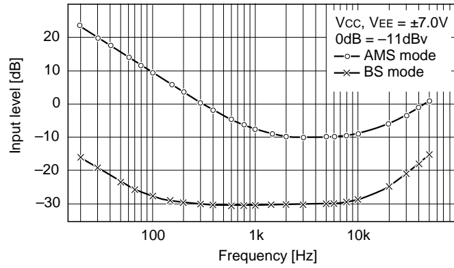
A.M./B.S mode frequency response
