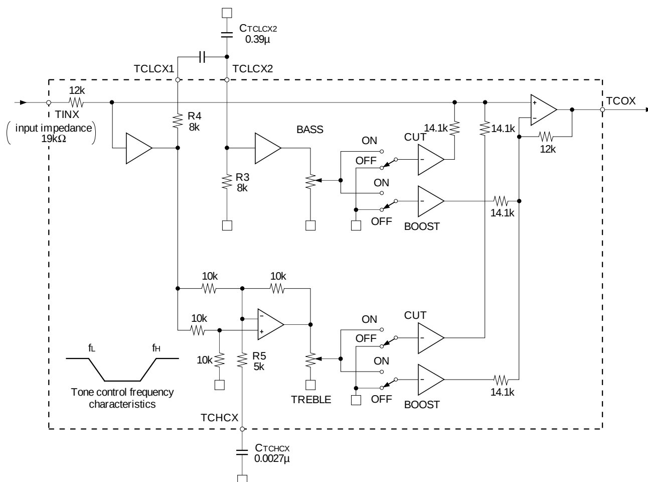
Fig. 4. Tone Control
