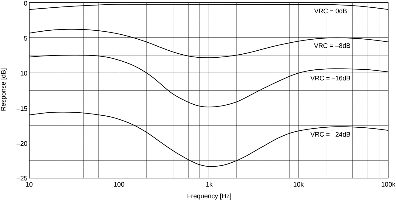
Loudness characteristics
