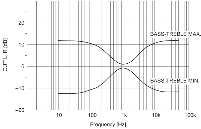
TONE characteristics
