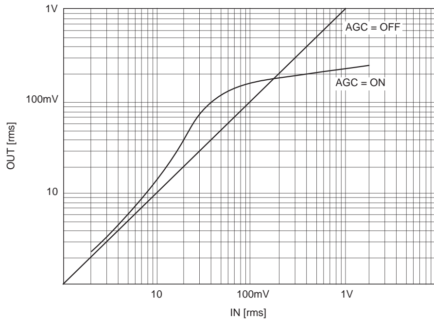
AGC characteristics
