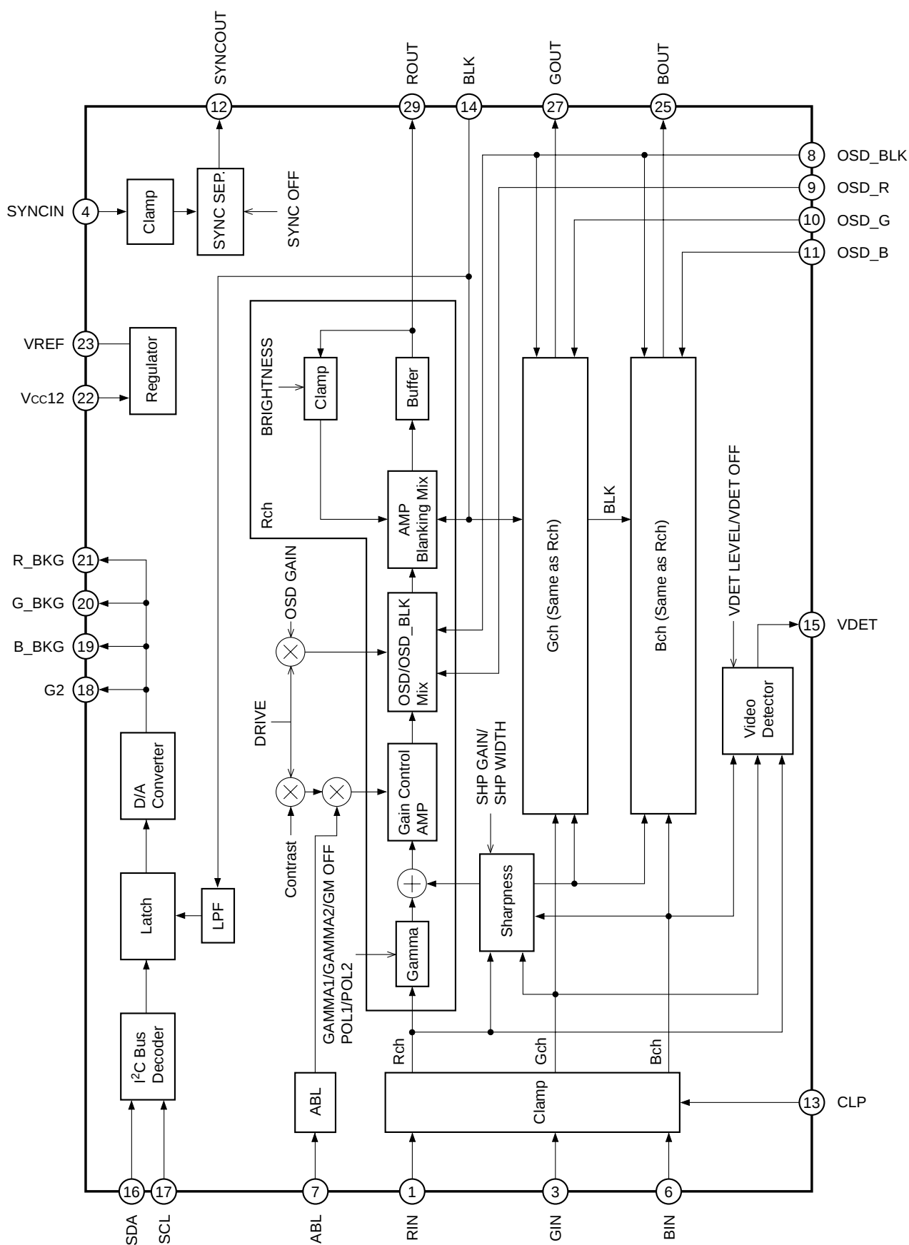
Block Diagram
