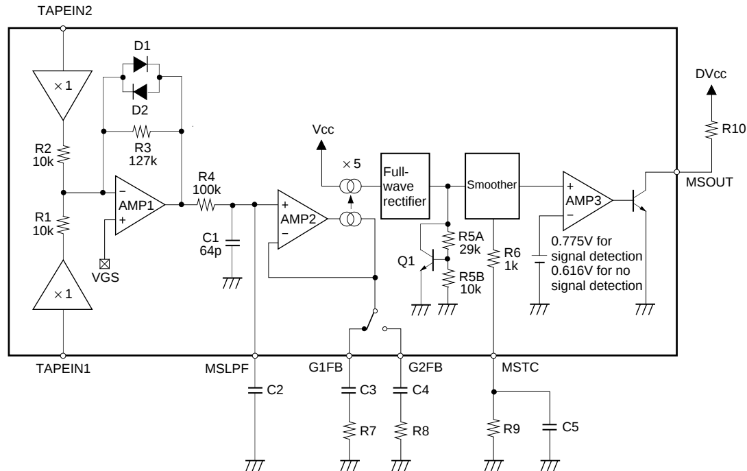
Fig. 5. Music sensor block diagram
