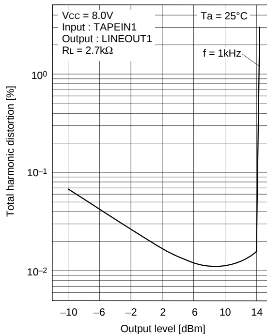
Total harmonic distortion (Line amplifier)
