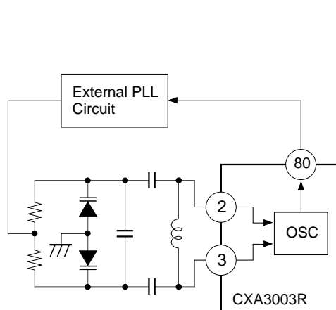
Fig. 11 Receive VCO
