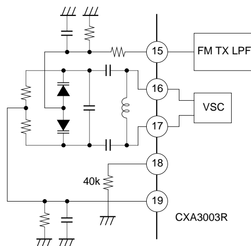
Fig. 12 Transmit VCO
