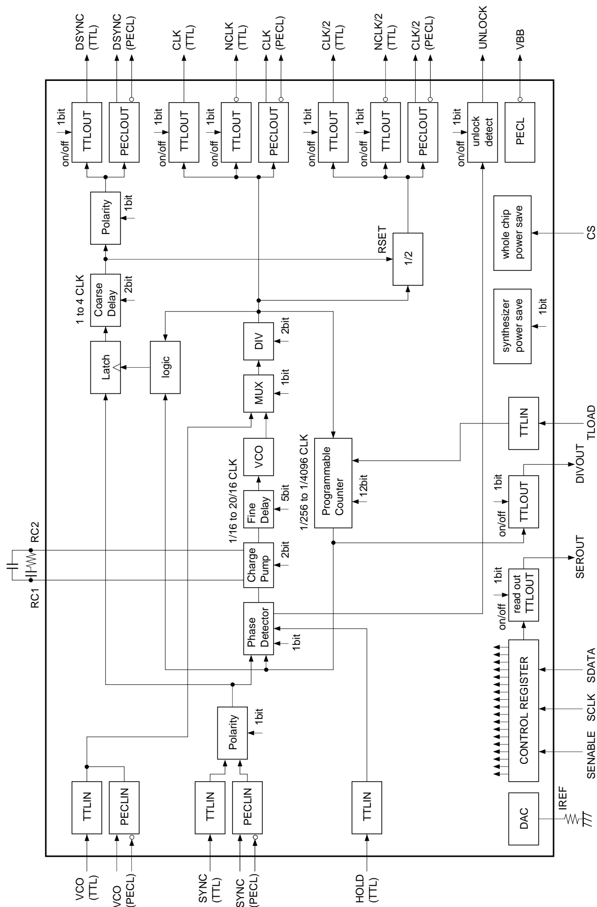
Block Diagram
