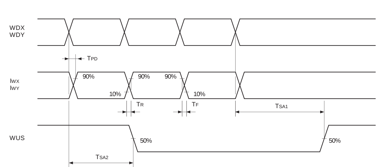
Timing Chart 2
