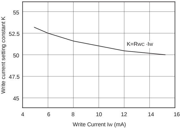
Fig.6 Write current setting constant vs. Write current
