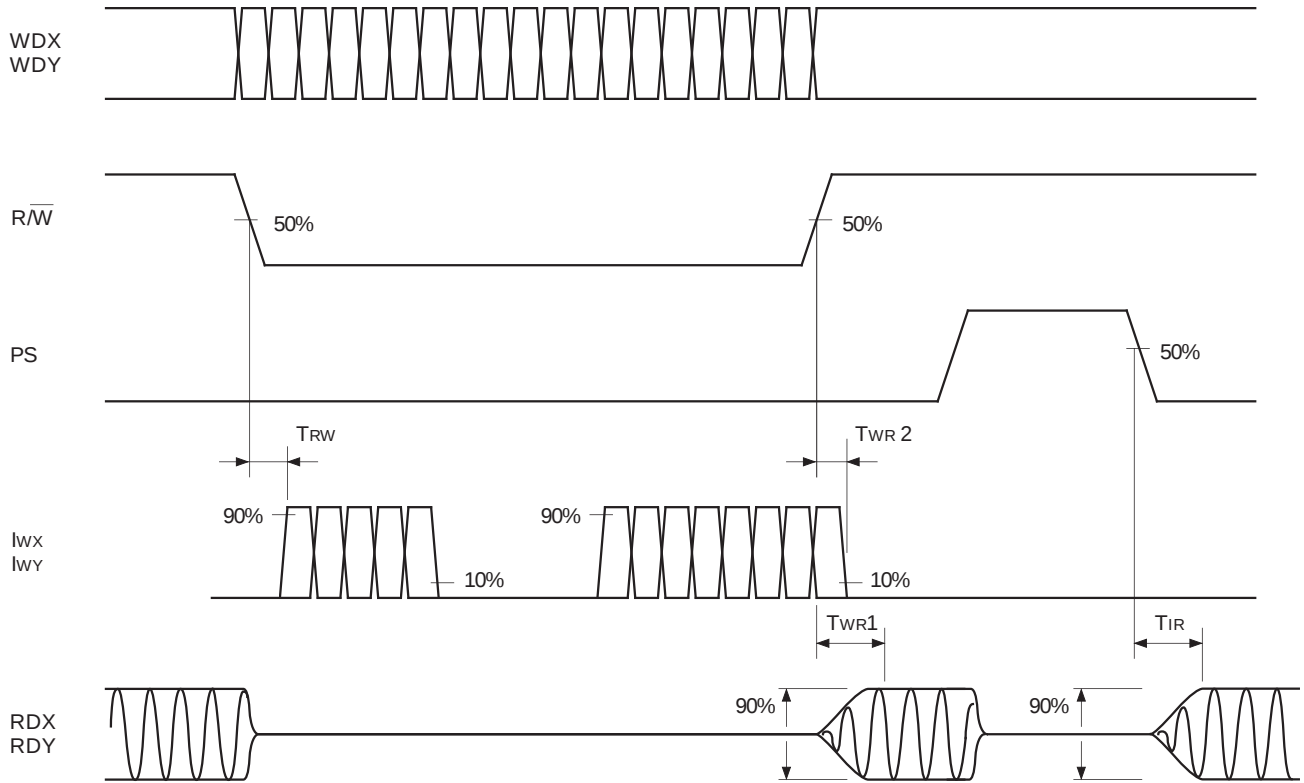
Timing Chart 1
