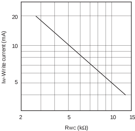
Fig.5 Write current vs. R wc
