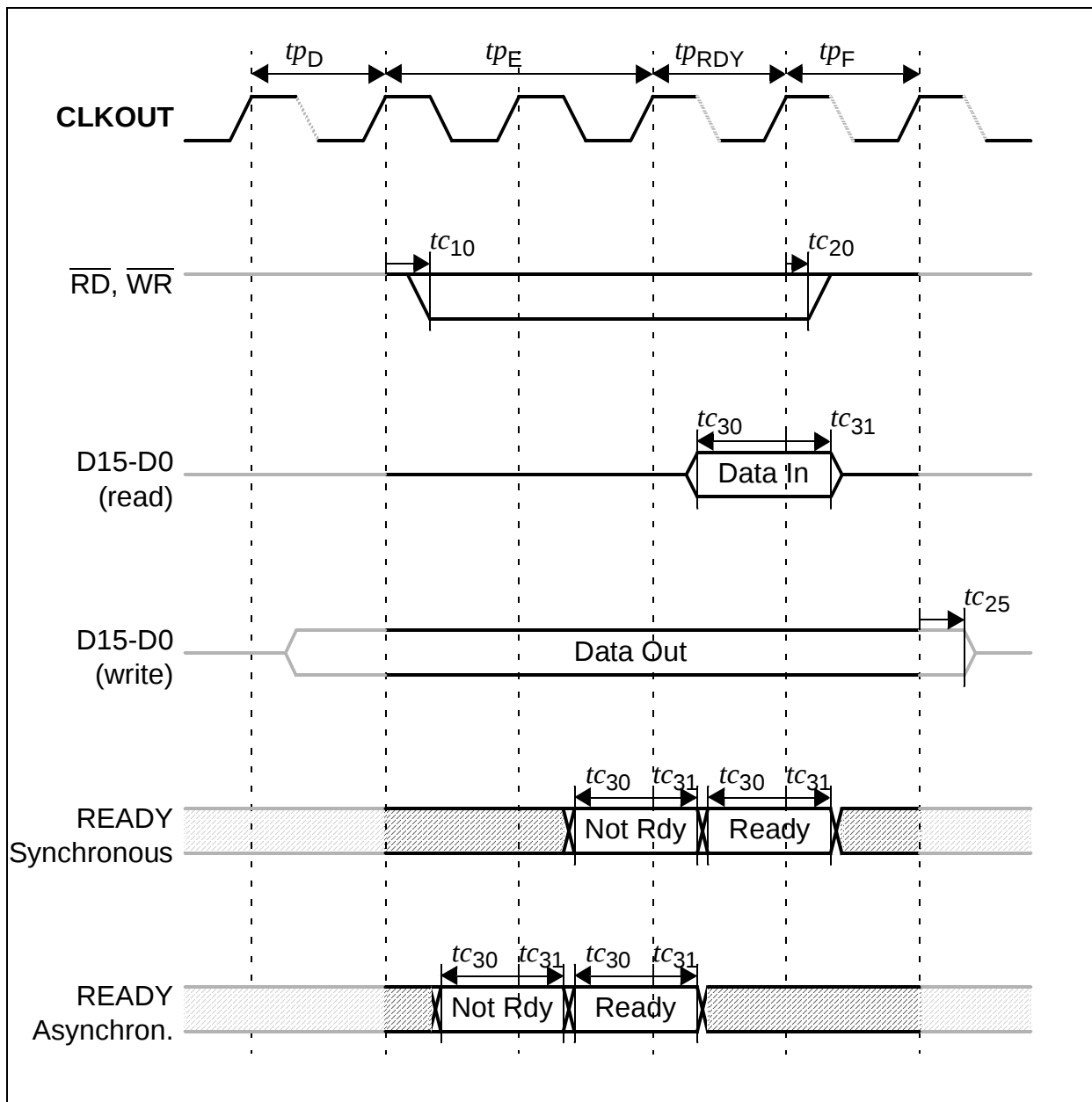
Figure 23 READY Timing
