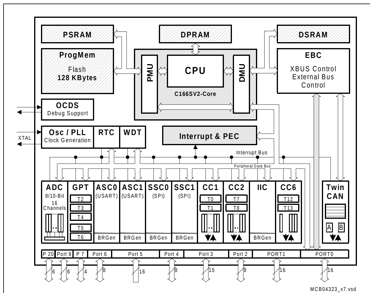
Figure 3 Block Diagram
