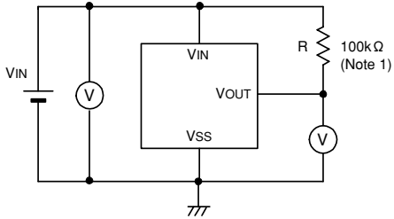
Circuit 1
