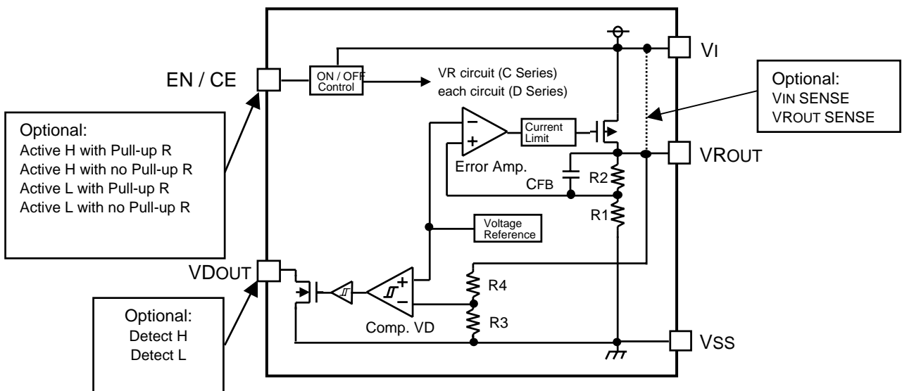
XC6413C, D Series
