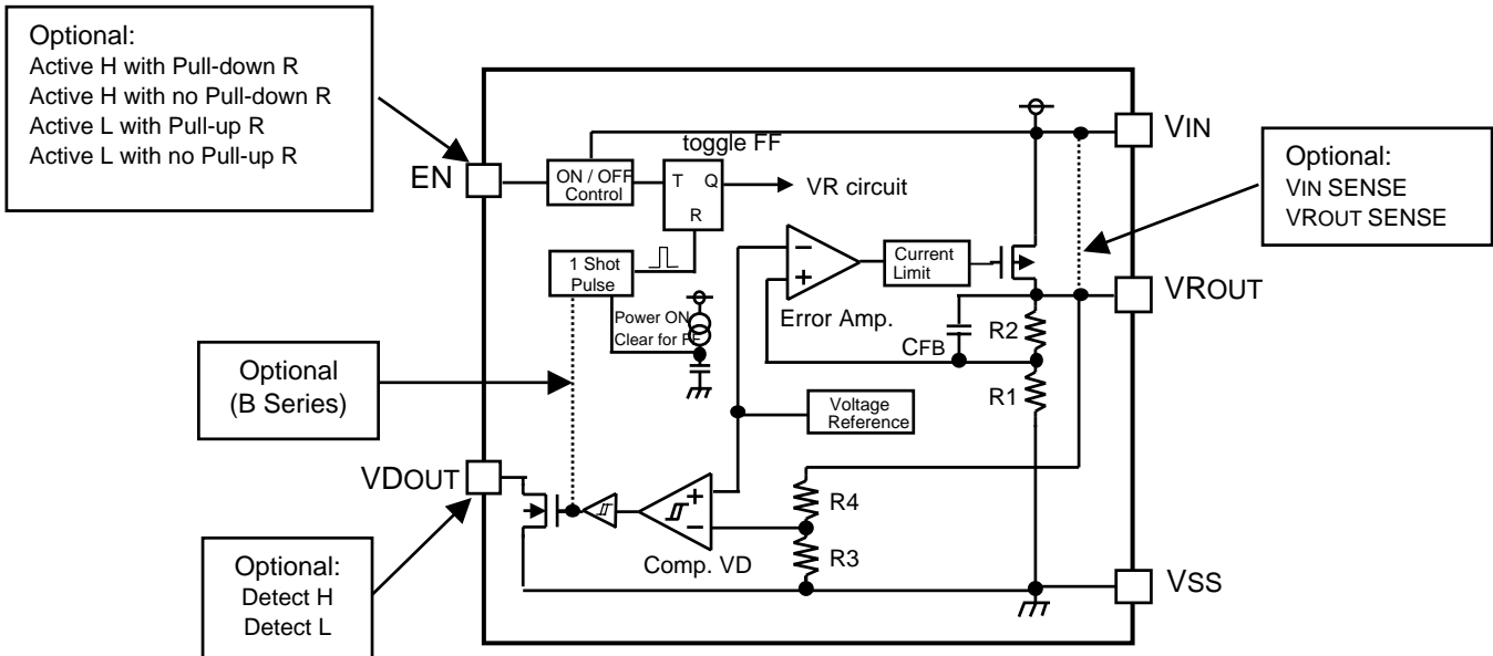
XC6413A, B Series
