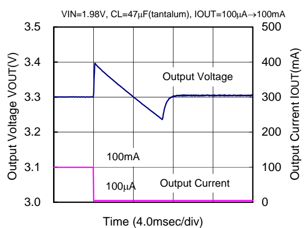
XC9104D092MR(PWM/PFM,180kHz,3.3V)
