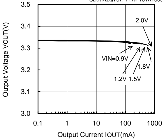
XC9103D095MR (PWM,500kHz,3.3V)
