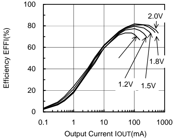
XC9103D095MR (PWM,500kHz,3.3V)
