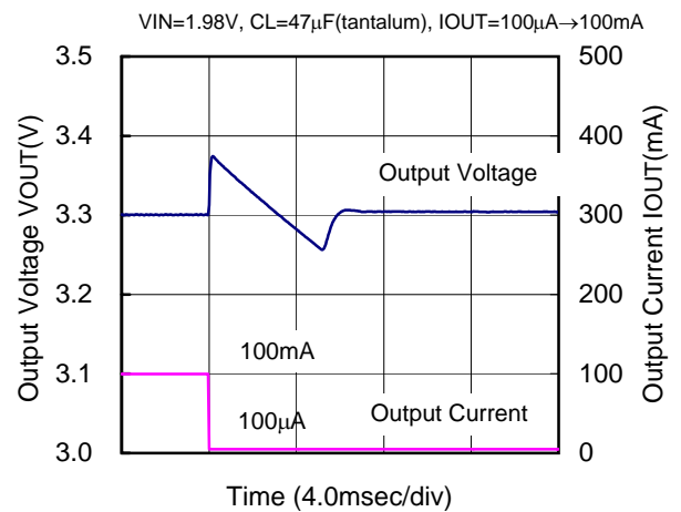
XC9103D092MR(PWM,180kHz,3.3V)
