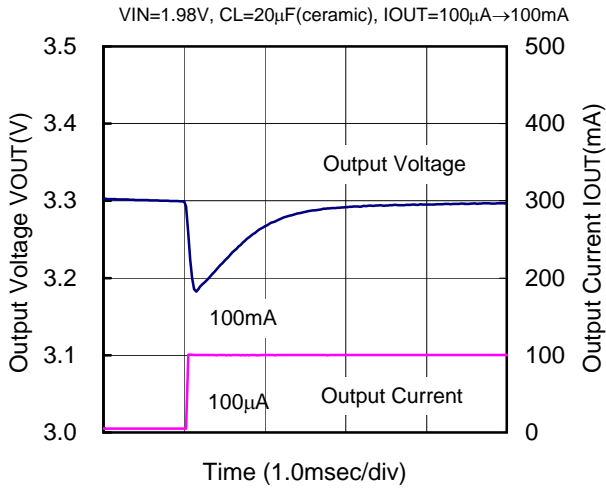
XC9104D093MR(PWM/PFM,300kHz,3.3V)
