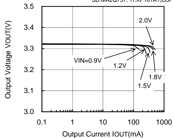
XC9104D092MR (PWM/PFM,180kHz,3.3V)
