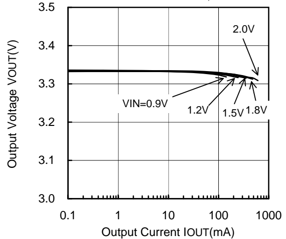
XC9104D095MR (PWM/PFM,500kHz,3.3V)
