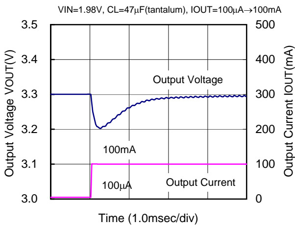
XC9103D092MR(PWM,180kHz,3.3V)
