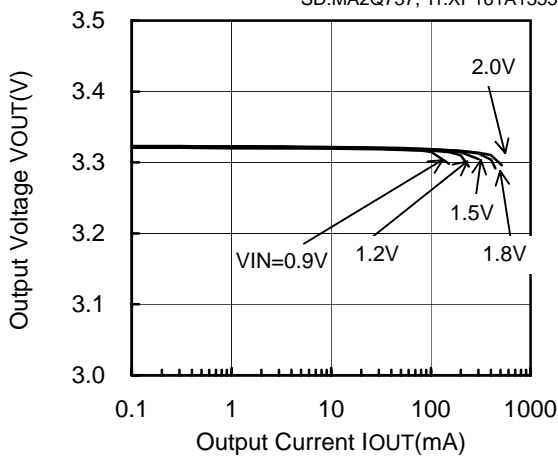
XC9103D092MR (PWM,180kHz,3.3V)
