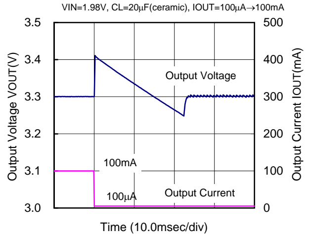
XC9104D093MR(PWM/PFM,300kHz,3.3V)
