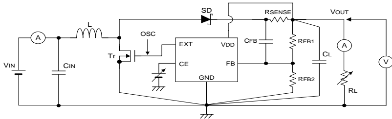
CIRCUIT ①
