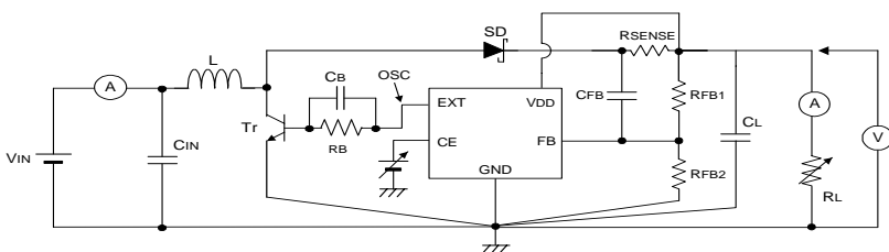
CIRCUIT ③
