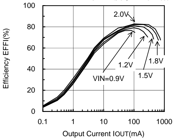
XC9103D093MR (PWM,300kHz,3.3V)
