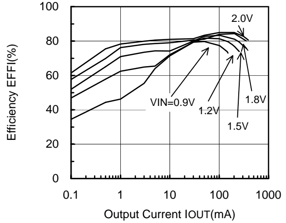
XC9104D092MR (PWM/PFM,180kHz,3.3V)
