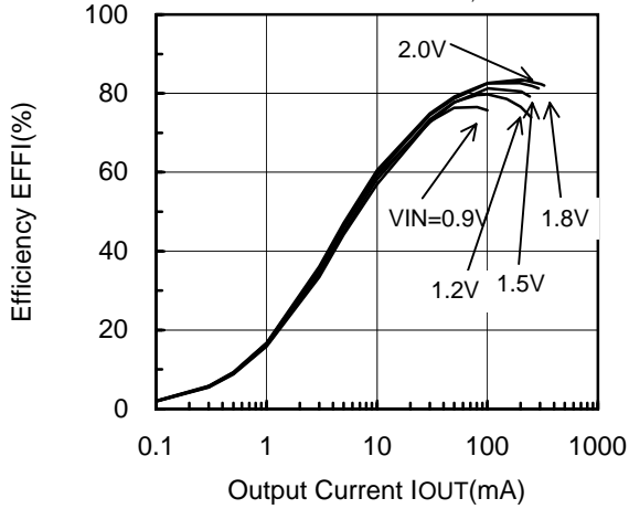
XC9103D092MR (PWM,180kHz,3.3V)
