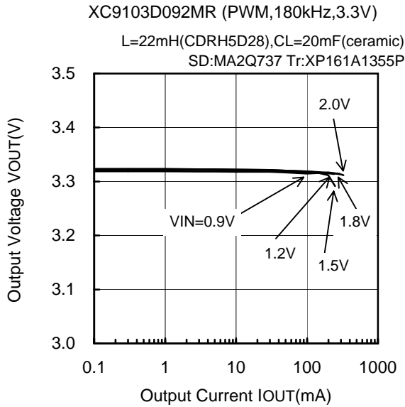
(1) Output Voltage vs. Output Current
