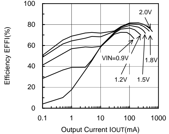
XC9104D095MR (PWM/PFM,500kHz,3.3V)
