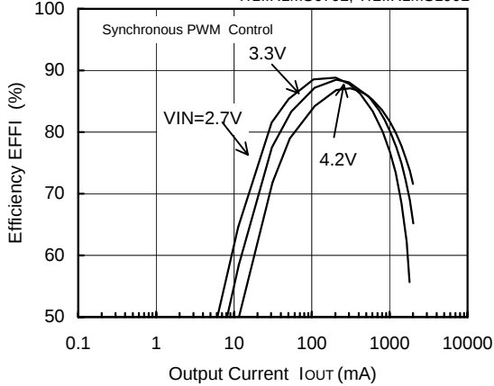
FOSC=300kHz, V_{OUT}=5.0V
