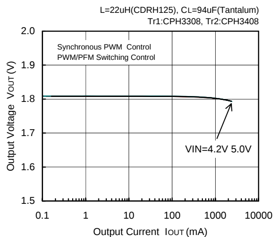
FOSC=180kHz, V_{OUT}=1.8V
