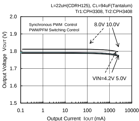
FOSC=300kHz, V_{OUT}=1.8V
