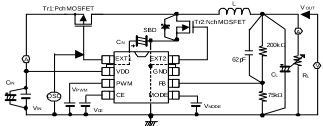
Circuit 4
