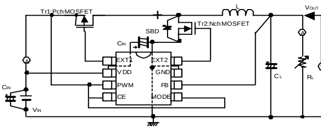
Circuit 5
