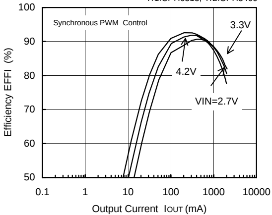
FOSC=180kHz, V_{OUT}=1.2V
