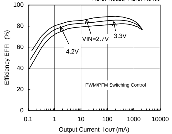
FOSC=180kHz, V_{OUT}=1.8V
