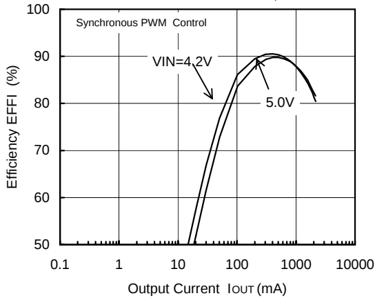
FOSC=180kHz, V_{OUT}=1.8V
