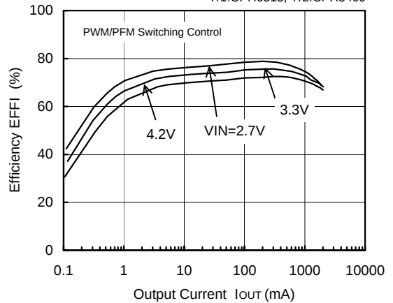
FOSC=180kHz, V_{OUT}=1.2V
