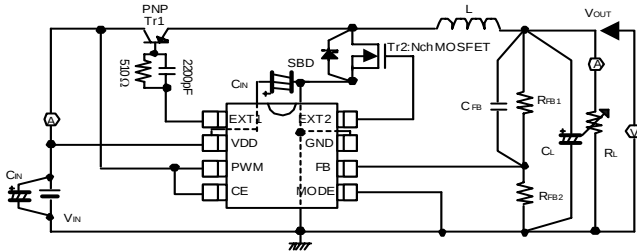
Circuit 3
