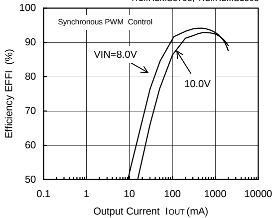
FOSC=180kHz, V_{OUT}=1.2V
