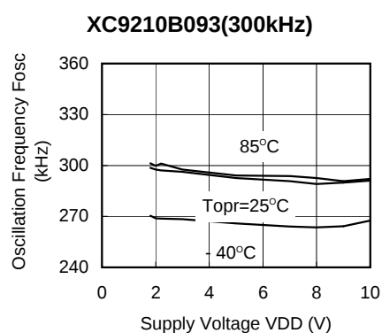
(13) Oscillation Frequency vs. Supply Voltage
