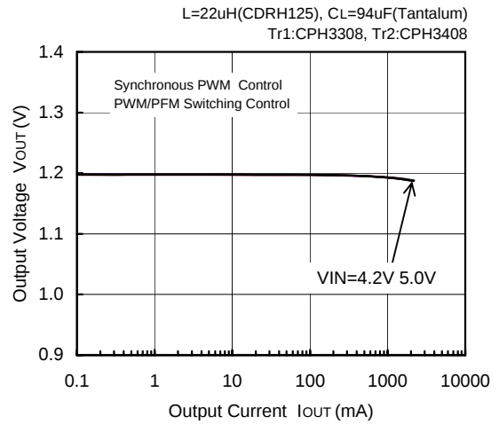
FOSC=180kHz, V_{OUT}=1.2V
