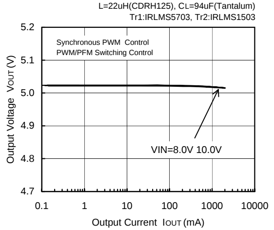
FOSC=300kHz, V_{OUT}=5.0V
