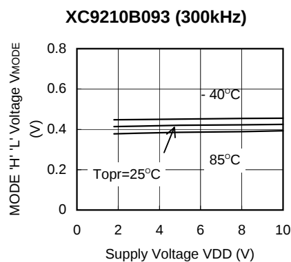
(12) MODE 'H' 'L' Voltage vs. Supply Voltage
