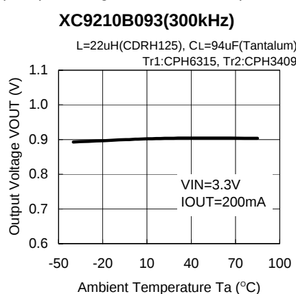
(19) Output Voltage vs. Ambient Temperature 2
