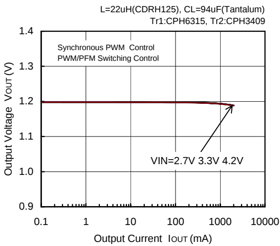
FOSC=180kHz, V_{OUT}=1.2V
