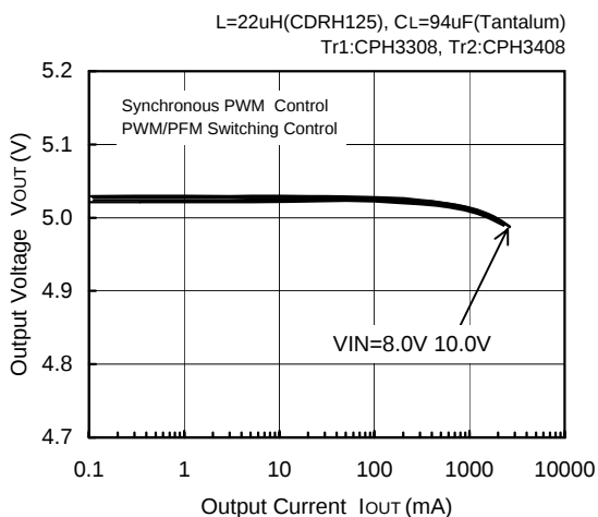
FOSC=300kHz, V_{OUT}=5.0V
