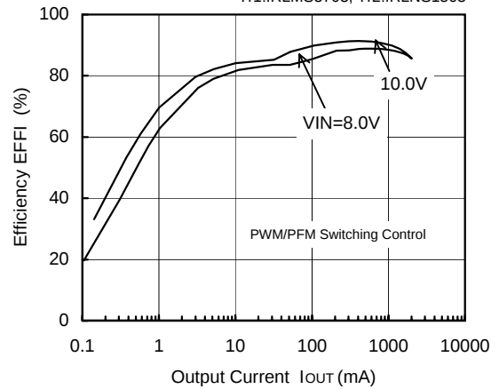
FOSC=180kHz, V_{OUT}=1.2V
