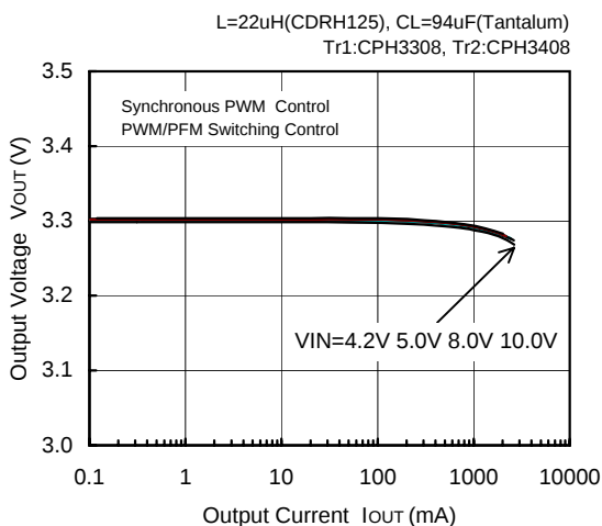
FOSC=300kHz, V_{OUT}=3.3V
