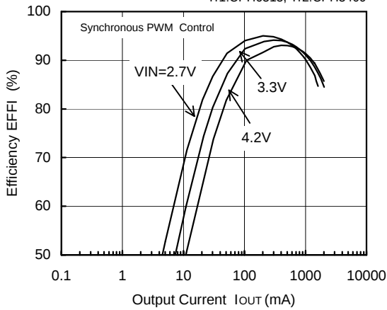
FOSC=180kHz, V_{OUT}=1.8V
