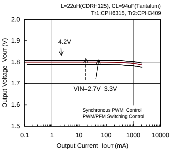
FOSC=180kHz, V_{OUT}=1.8V
