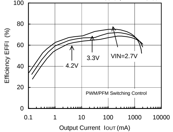
FOSC=300kHz, V_{OUT}=5.0V
