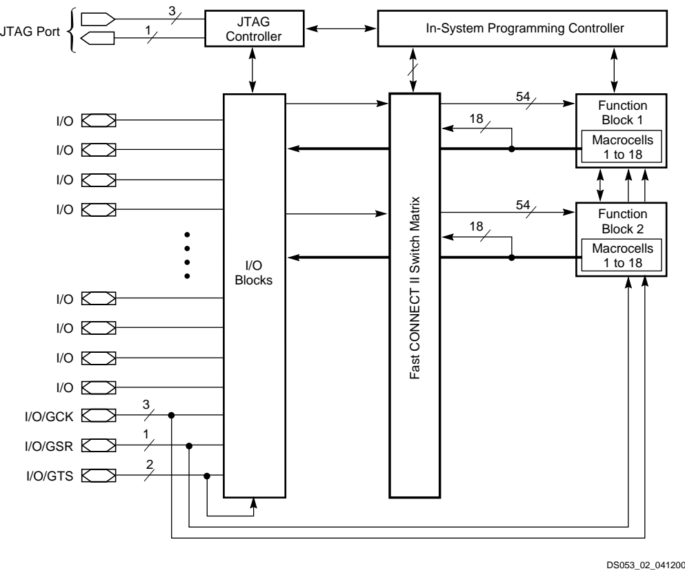
Figure 2: XC9536XV Architecture Function block outputs (indicated by the bold line) drive the I/O Blocks directly.
