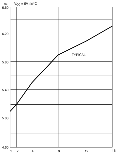
Figure 5: t_{PD\_PAL} vs Outputs Switching
