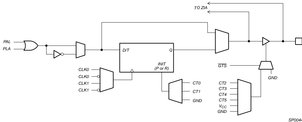
Figure 2: XCR5032 Macrocell Architecture
