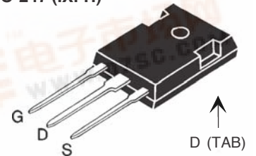
TO-247 (IXFH)
