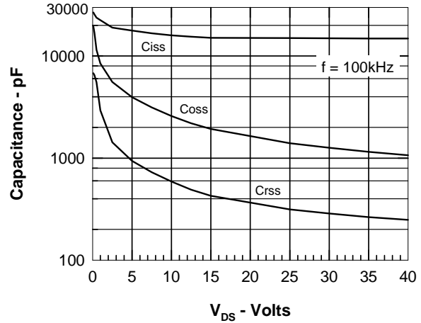
Figure 8. Capacitance Curves
