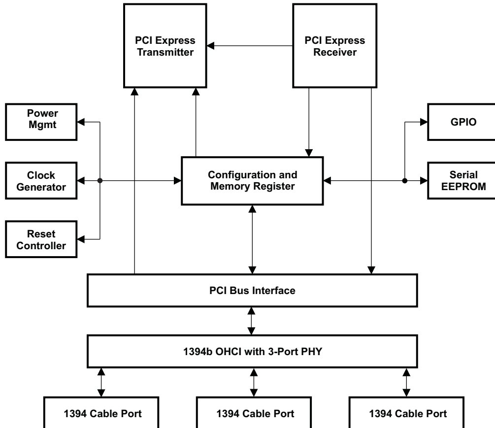
Figure 3-1. XIO2213B Block Diagram
