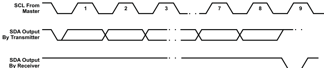
Figure 3-8. Serial-Bus Protocol Acknowledge
