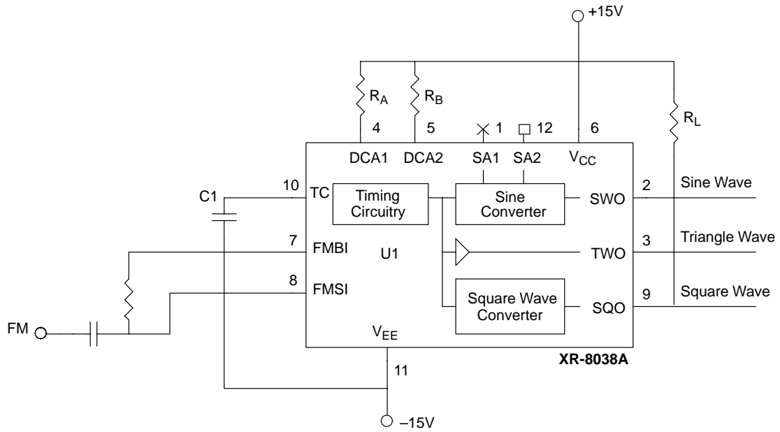
Figure 8. Frequency Modulator
