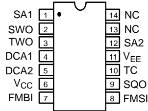
14 Lead PDIP (0.300")
