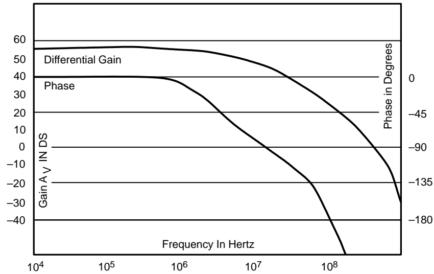
Figure 5. Preamp Gain/Phase Characteristics
