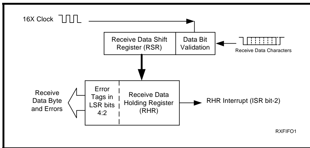
FIGURE 9. RECEIVER OPERATION IN NON-FIFO MODE
