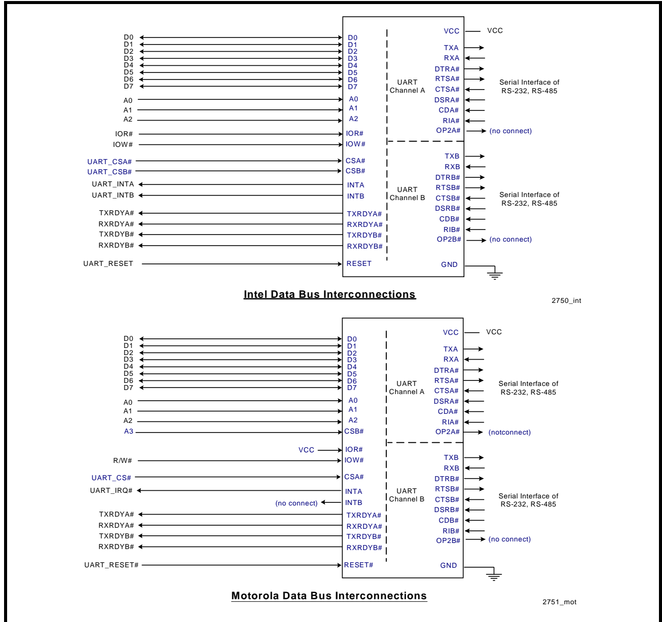
FIGURE 3. XR16L2751 TYPICAL INTEL/MOTOROLA DATA BUS INTERCONNECTIONS
