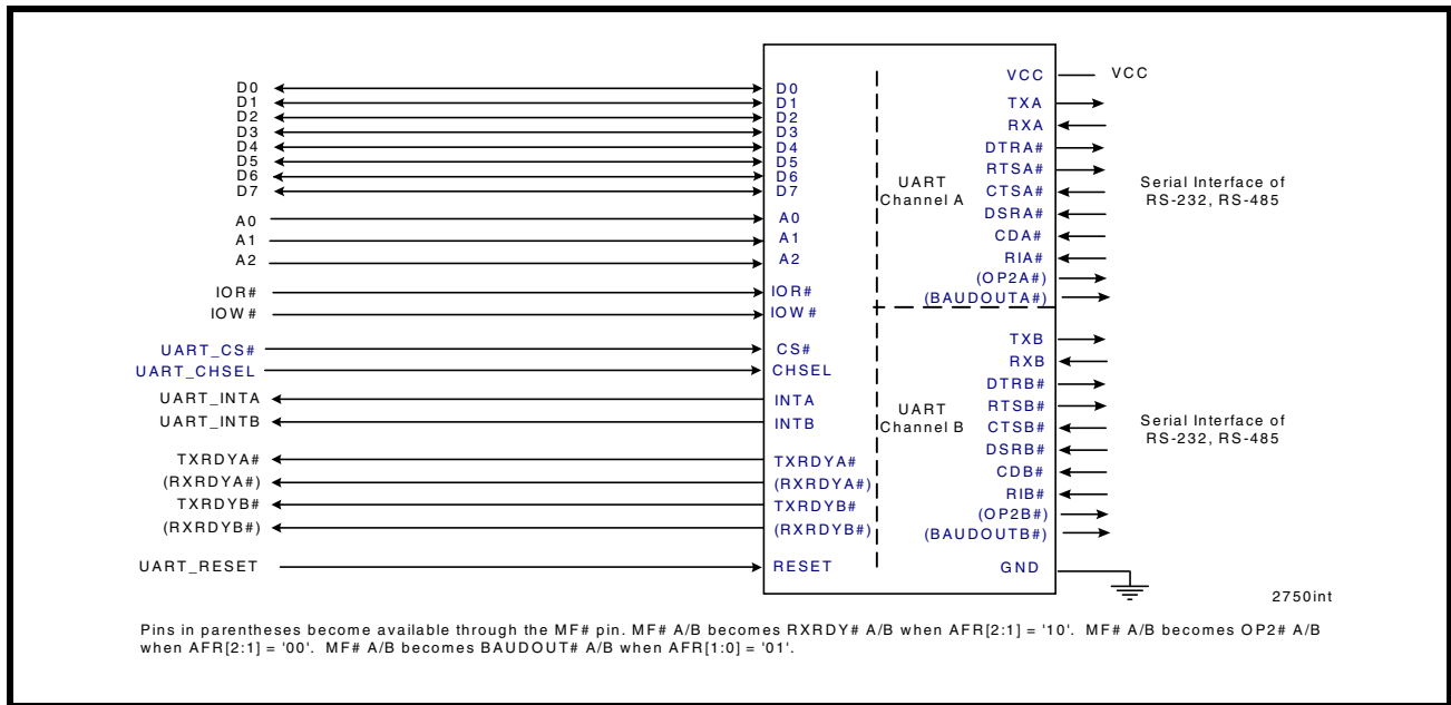
FIGURE 3. XR16L2752 DATA BUS INTERCONNECTIONS
