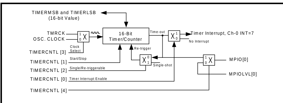
FIGURE 5. TIMER/COUNTER CIRCUIT.
