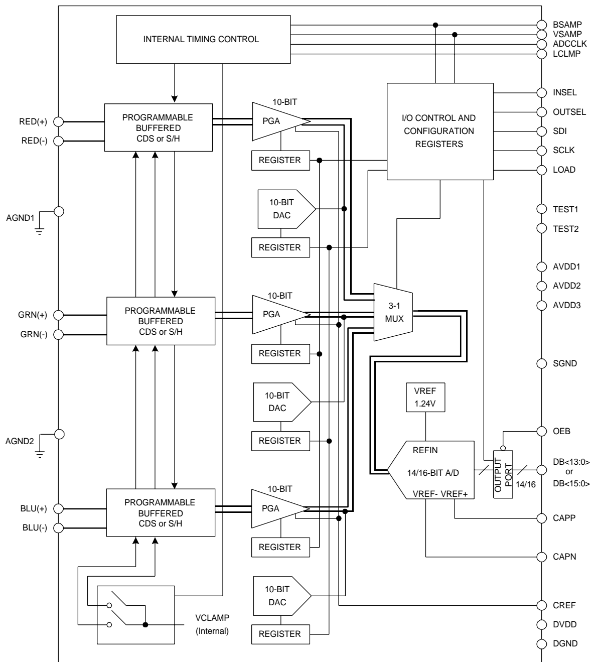
Figure 1. Block Diagram
