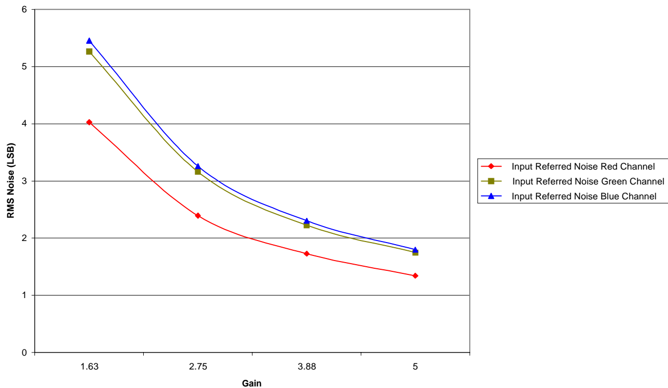
Graph 6. XRD9814 3-Channel CDS Pixel Clamp Input Referred Noise vs. Gain
