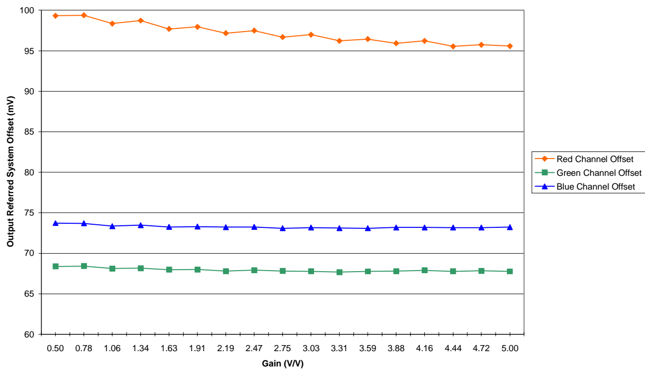
Graph 8. XRD9814 /9816 3-Channel CDS Pixel Clamp System Offset vs. Gain
