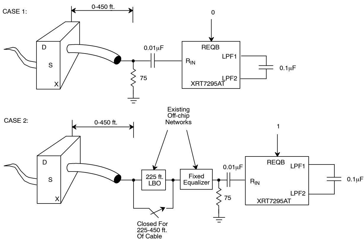
Figure 3. Receiver Configurations
