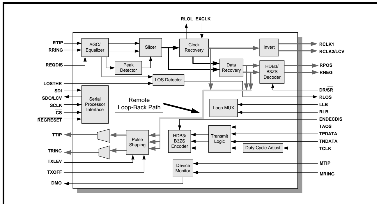
FIGURE 31. THE REMOTE LOOP-BACK PATH IN THE XRT73L00A
