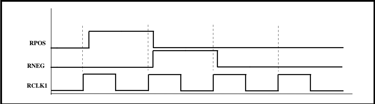
FIGURE 25. HOW THE XRT73L00A OUTPUTS DATA ON THE RPOS AND RNEG OUTPUT PINS
