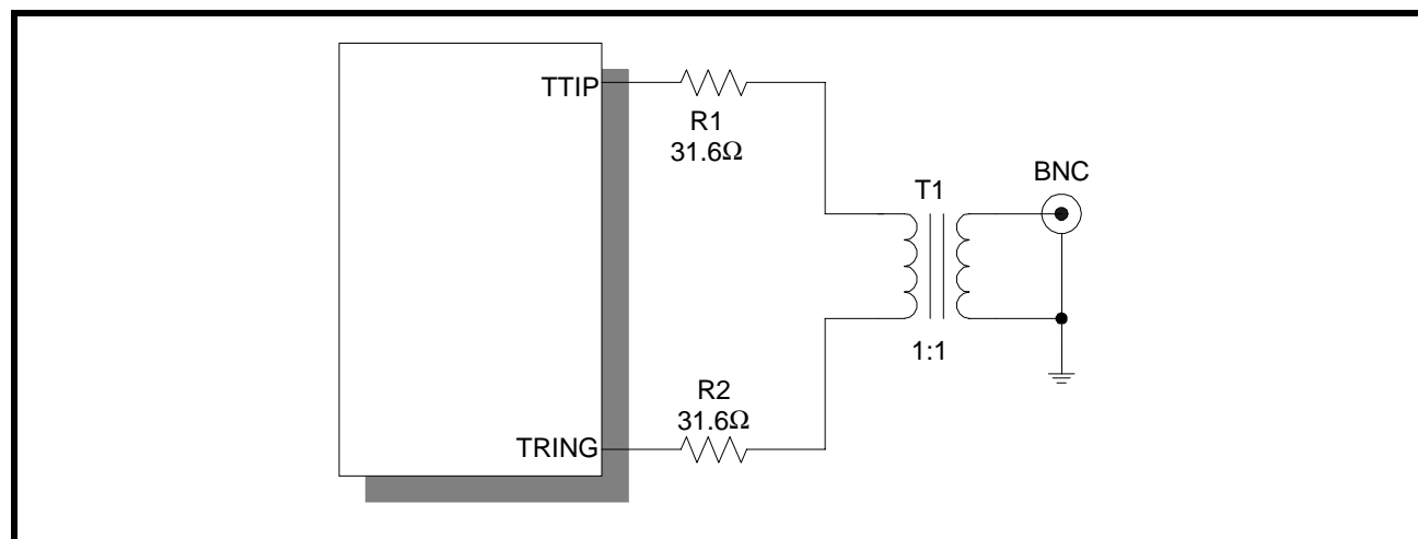
FIGURE 16. RECOMMENDED SCHEMATIC FOR INTERFACING THE TRANSMIT SECTION OF THE XRT73L00A TO THE LINE
