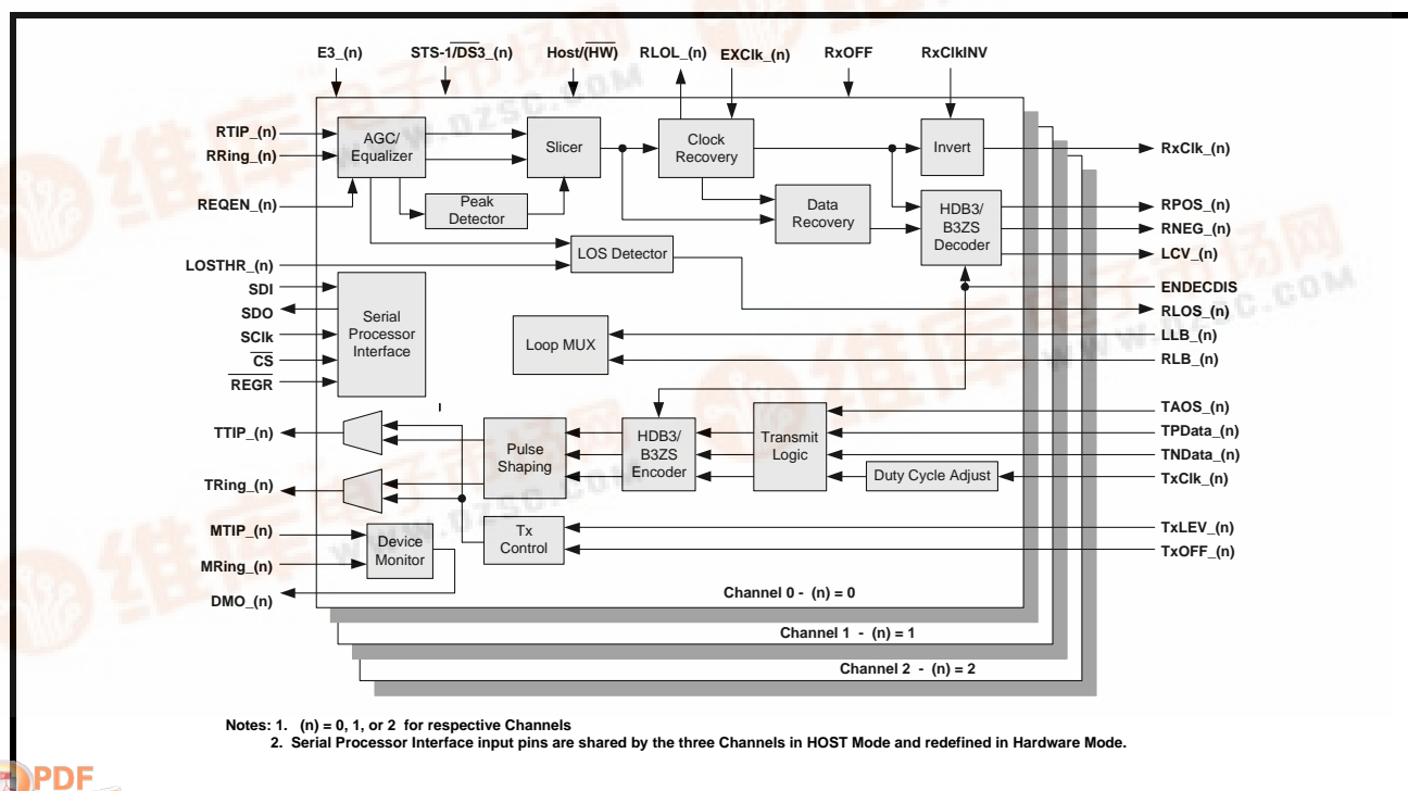
FIGURE 1. XRT73LC03A BLOCK DIAGRAM
