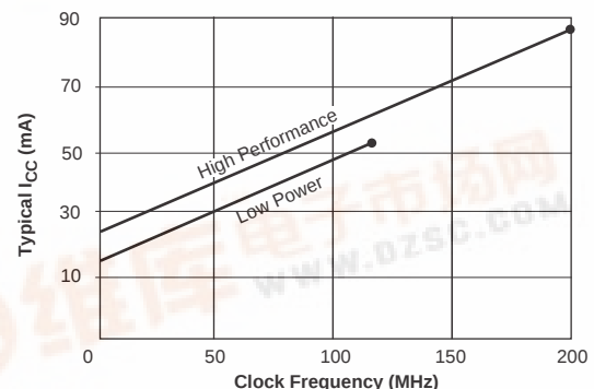
Figure 1: Typical I_{CC} vs. Frequency for XC9572XV
