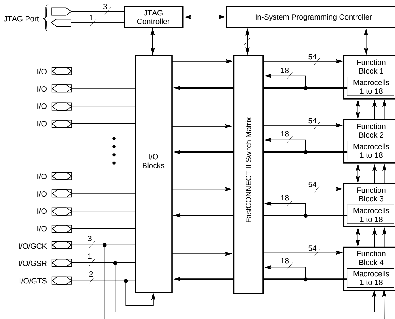
Figure 2: XC9572XV Architecture
