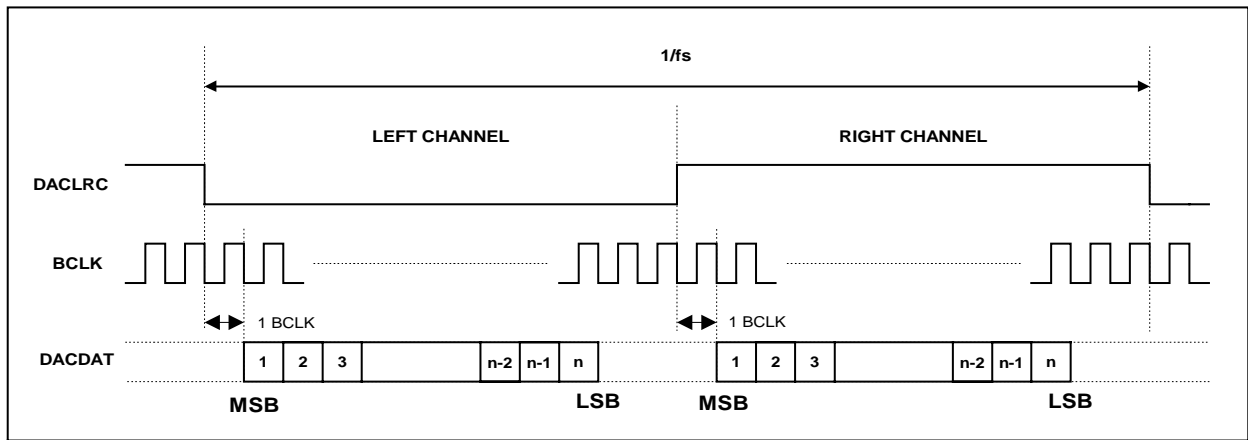
Figure 14 I2S Mode
