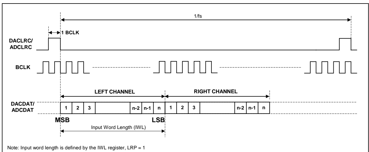
Figure 28 DSP Mode
