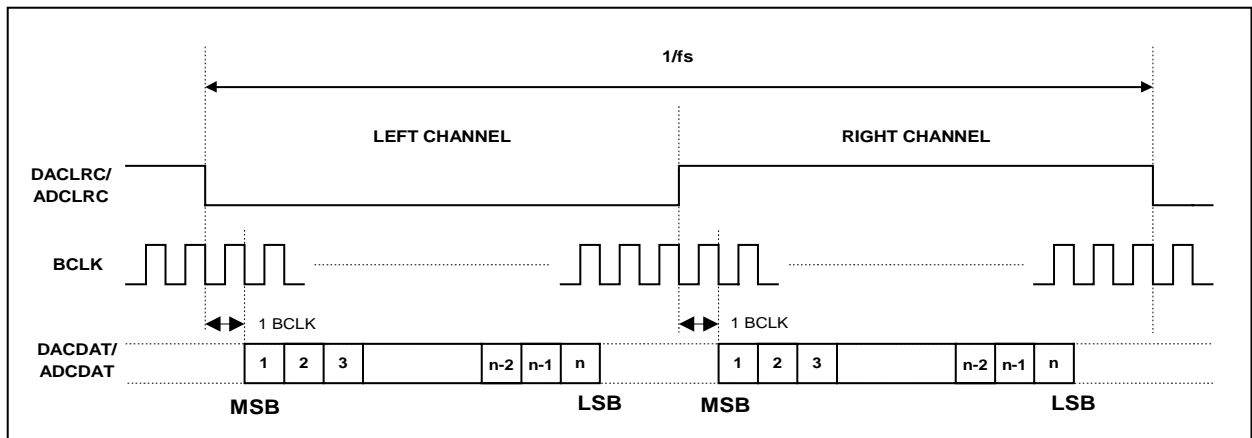
Figure 26 I2S Mode
