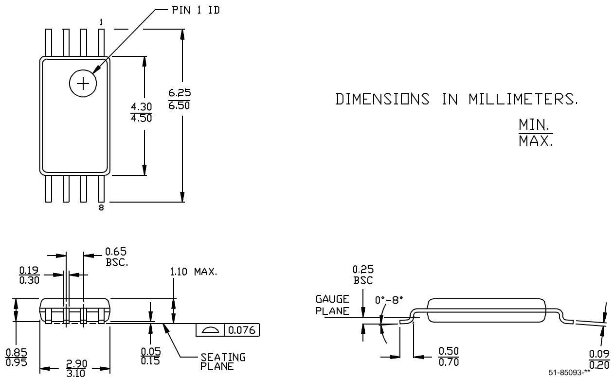
8-pin Thin Shrink Small Outline Package (4.40 MM Body) Z8
