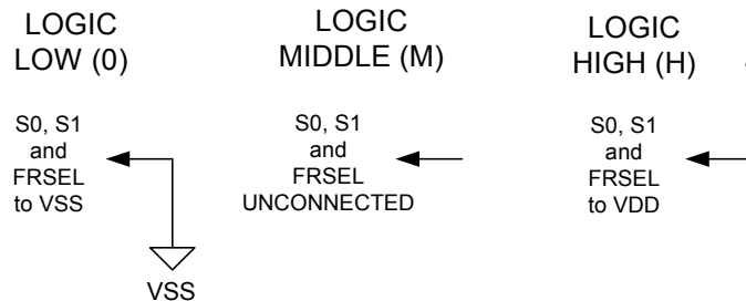
Figure 1. 3-Level Logic
