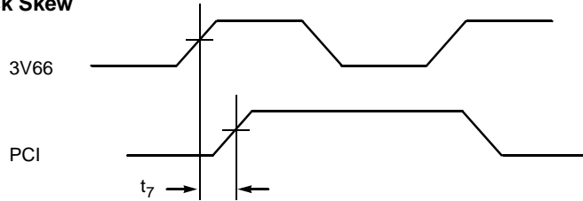
3V66-PCI Clock Skew
