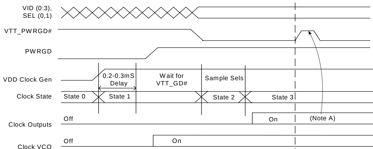
Figure 6. VTT_PWGD# Timing Diagram (With Advanced PIII Processor SelP4 K7 = 1 ) [31]
