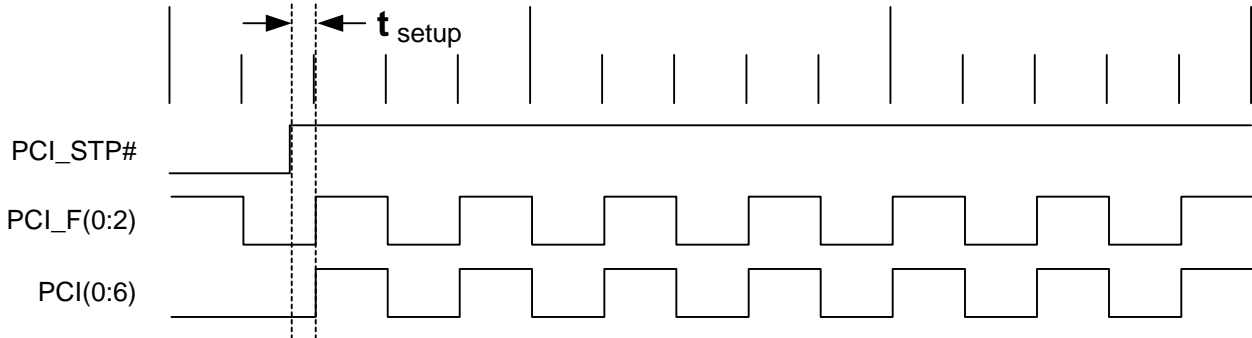
Figure 4. Deassertion PCI_STP# Waveform [7]
