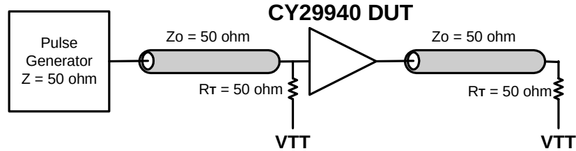
Figure 1. LVC MOS_CLK CY29940 Test Reference for V_{CC} = 3.3V and V_{CC} = 2.5V
