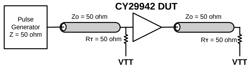
Figure 1. LVC MOS_CLK CY29942 Test Reference for V_{CC} = 3.3V and V_{CC} = 2.5V
