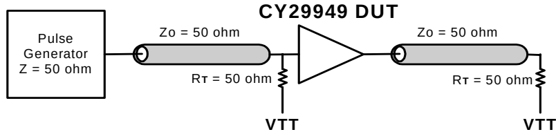
Figure 1. LVC MOS_CLK CY29949 Test Reference for V_{CC} = 3.3V and V_{CC} = 2.5V
