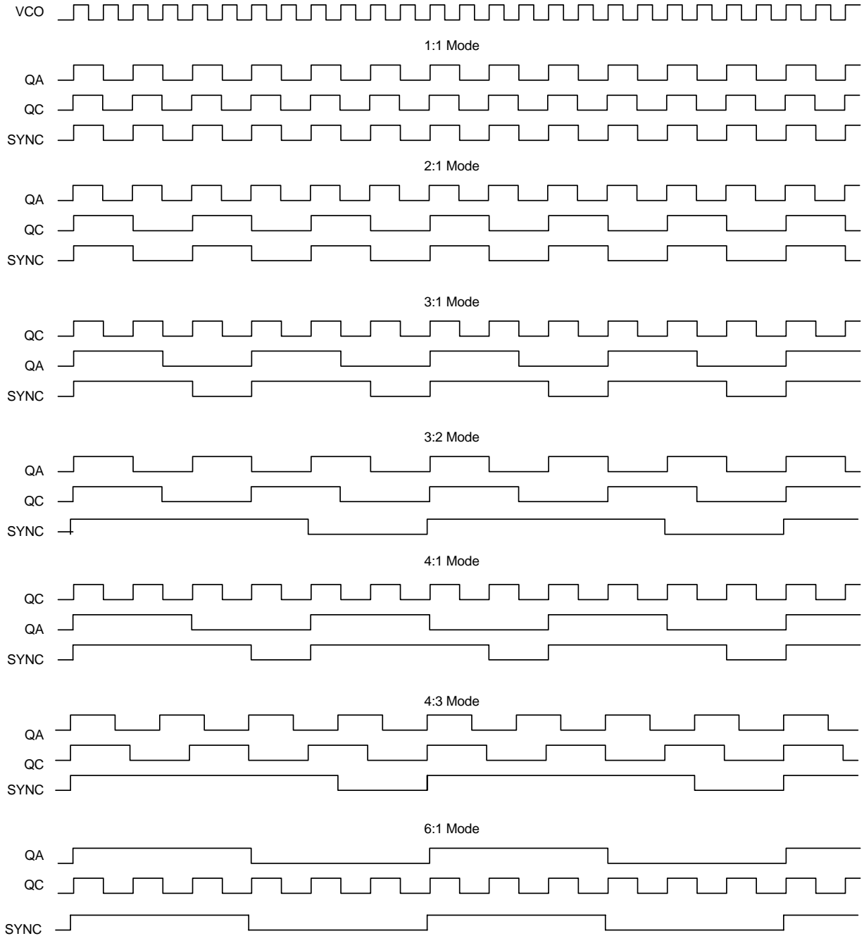
Figure 1. Timing Diagram
