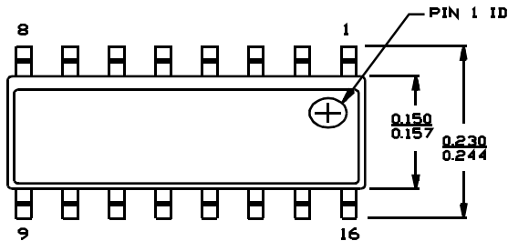
16-lead (150-mil) Molded SOIC S16
