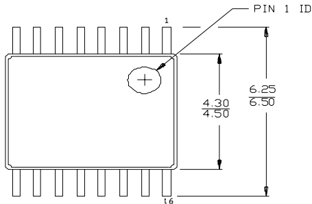
16-lead Thin Shrink Small Outline Package (4.40 MM Body) Z16
