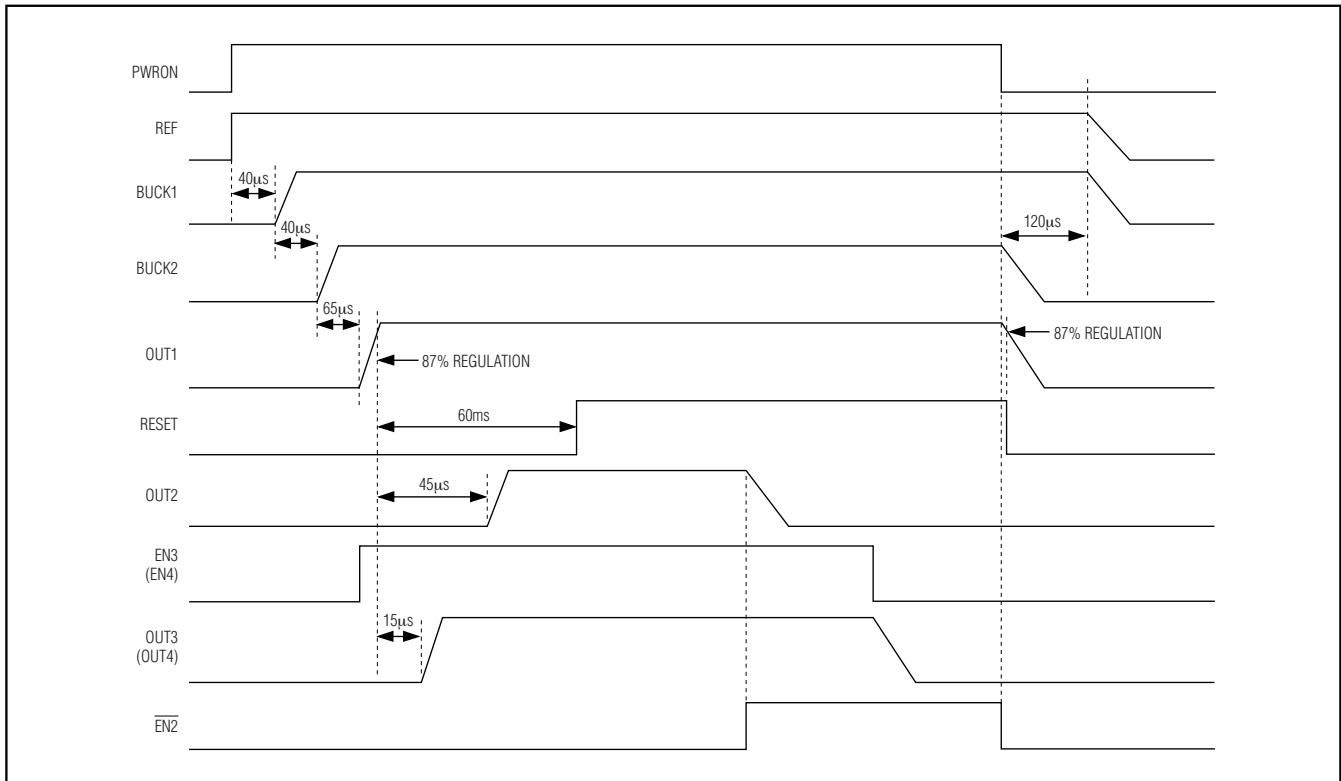
Figure 2. Power-On/Off Sequence Diagram
