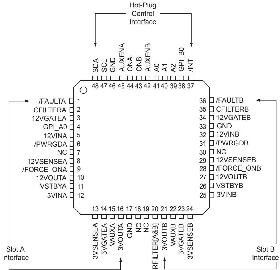
48-Pin TQFP
