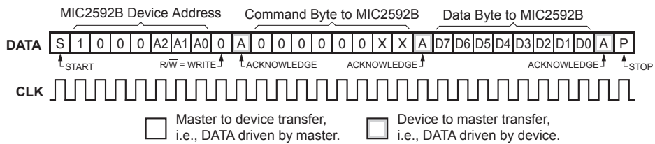
Figure 10. WRITE_BYTE Protocol
