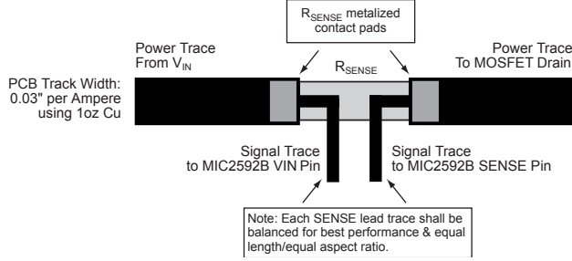
Figure 13. 4-Wire Kelvin Sense Connections for R_{SENSE}
